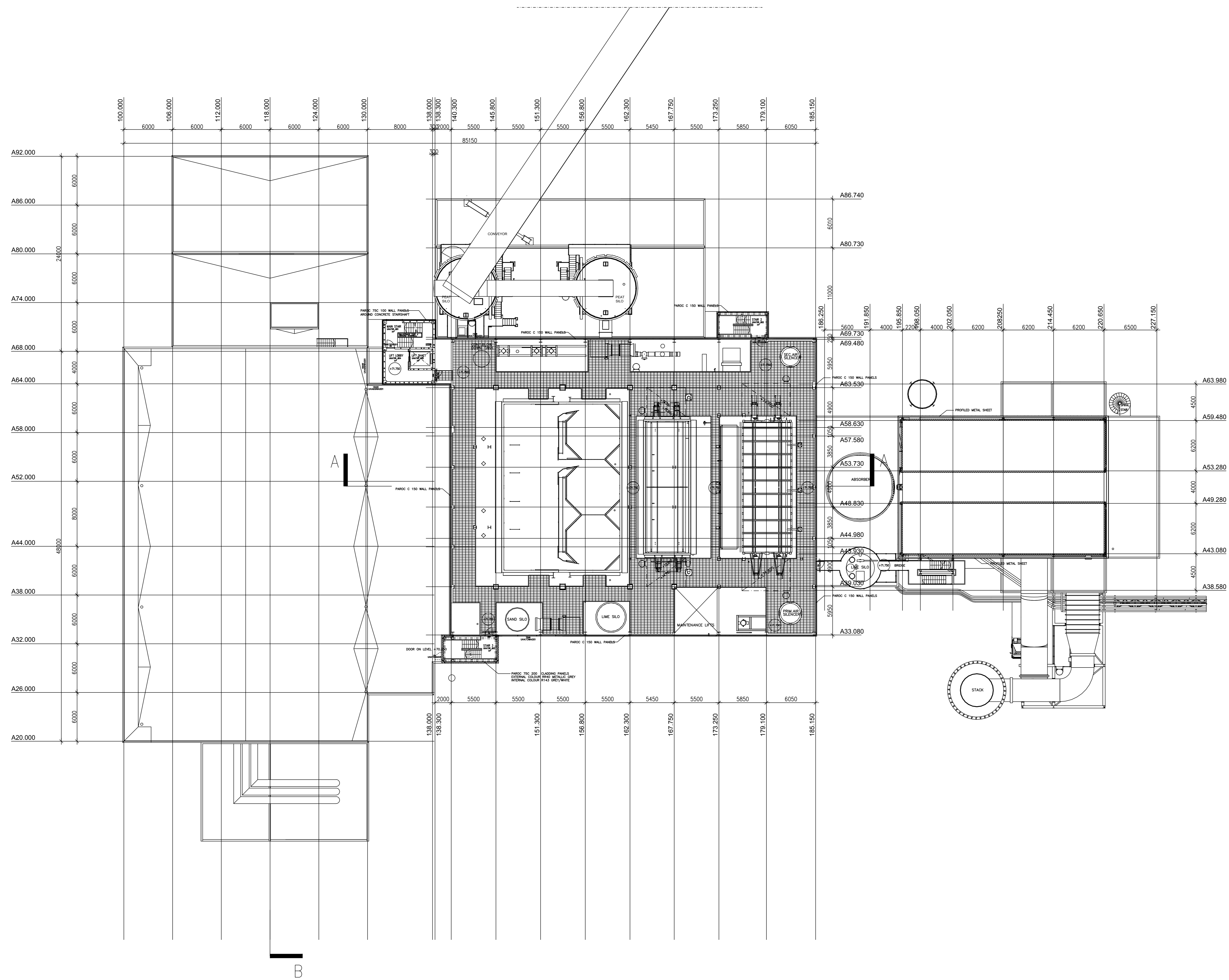
PLAN @ LEVEL +71.750m
